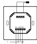
Figure 8. Wiring (1)
